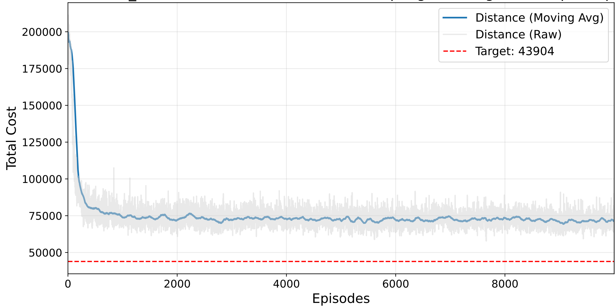
Final NO_MASK Masked AutoRL-SOP (Resampling) Training - kro124p.3.sop
